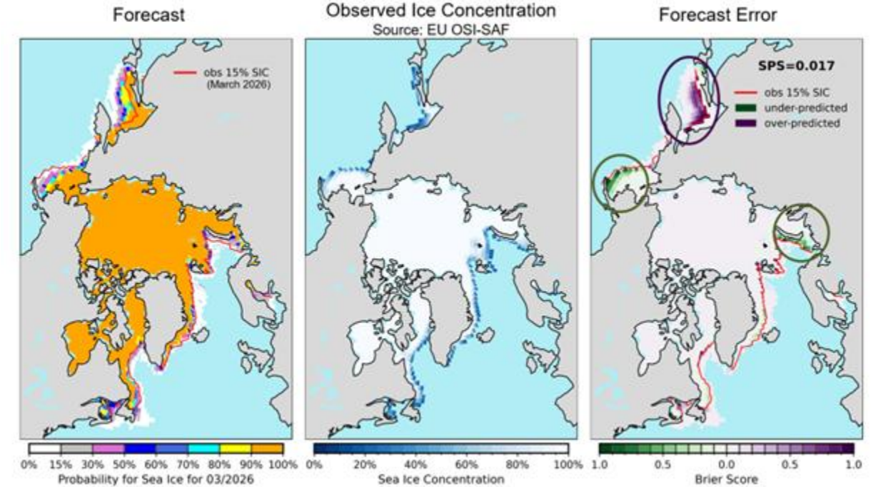
Figure 13: Verification of CanSIPSv3 probabilistic forecast for March 2026: Probability of ice concentration exceeding 15%
