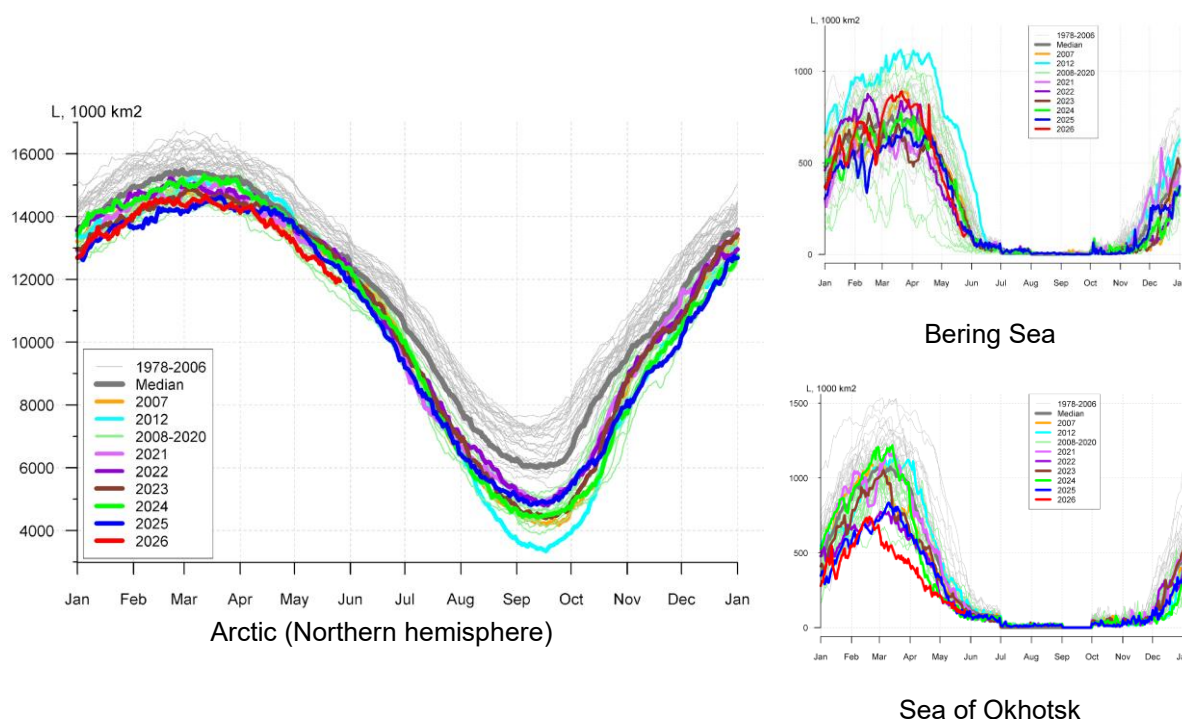
Figure 11: Arctic (Northern Hemisphere), Bering and Sea of Okhotsk daily sea-ice extent for October 1978 - May 2026. Graphics produced by the AARI. Data source: NSIDC.
