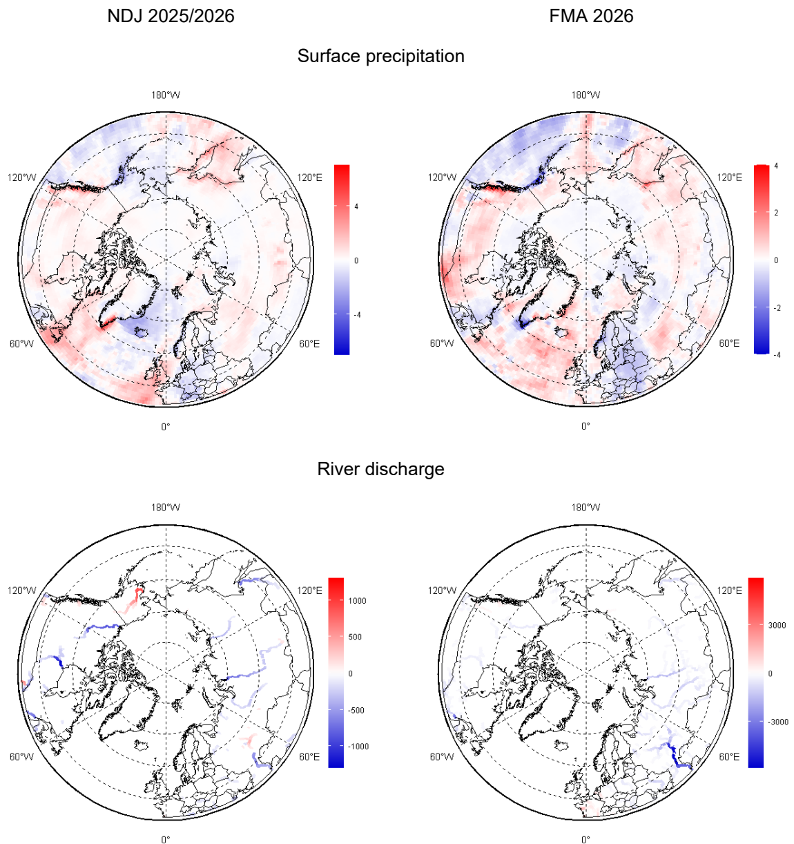
Figure 7 – November-January 2025/2026 and February – April 2026 surface precipitation (top) and river discharge (bottom) anomalies (ref. 1991-2020). Maps produced by the AARI. Data source: CCCS ERA5 and RA5-GloFAS.
