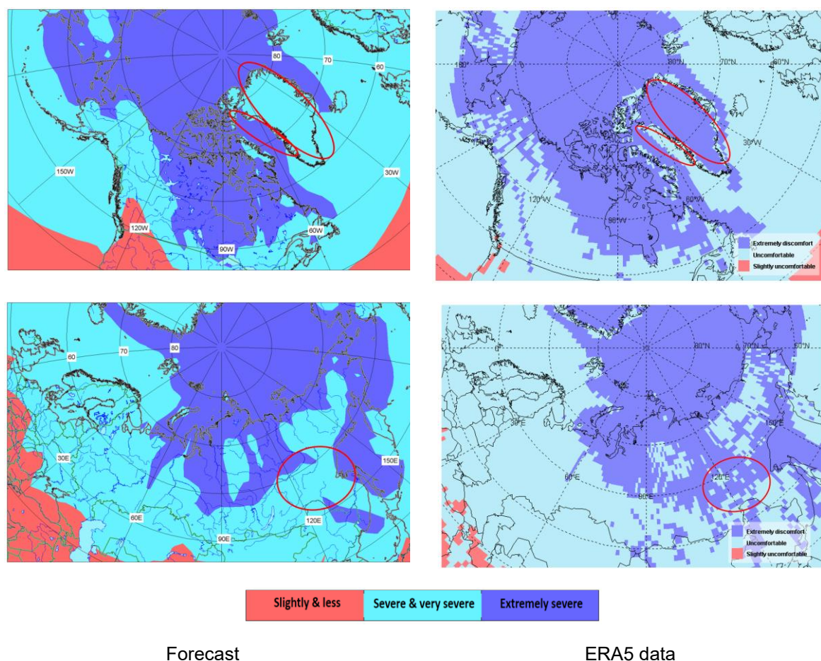
Figure 18: Bodman's index (S) of weather severity forecast (left) and ERA5 reanalysis estimate (right) for December 2025 – February 2026. Maps produced by the AARI and Hydrometcenter Russia. Data source: Hydrometcenter Russia and CCCS ERA5.
