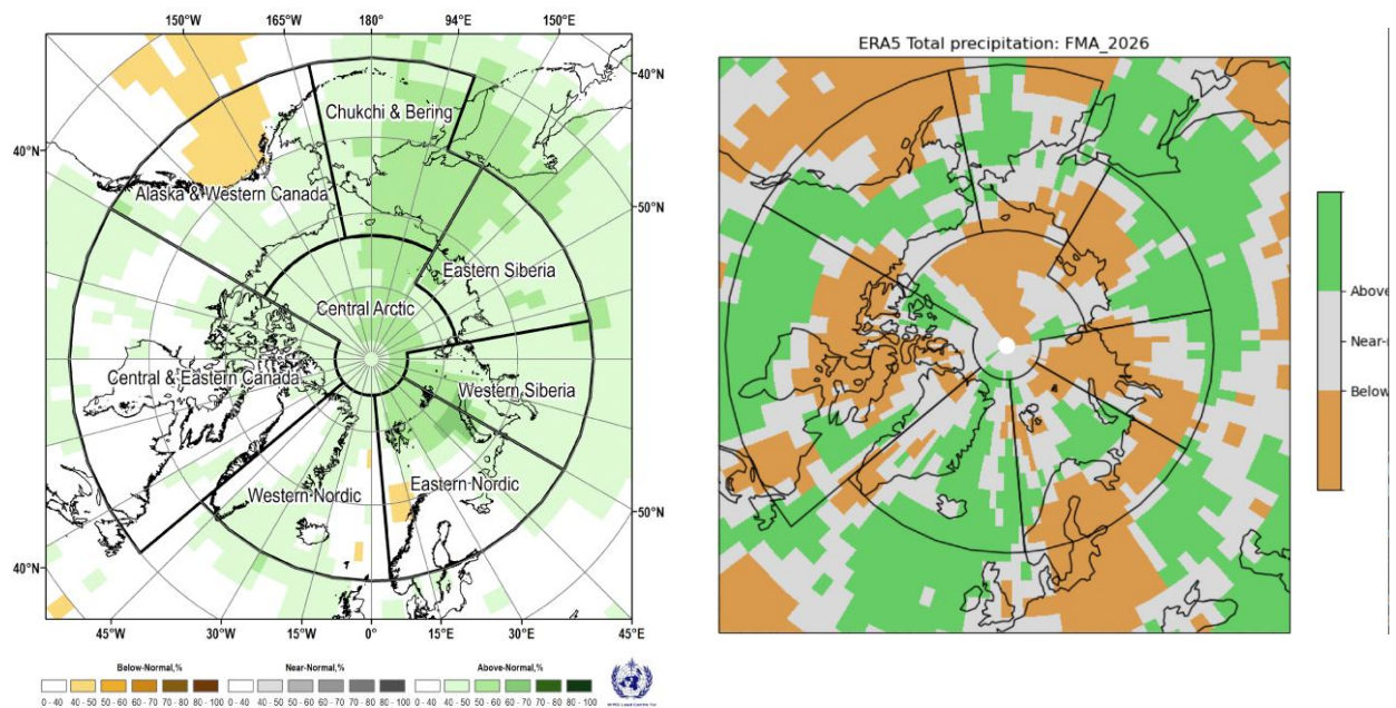
Figure 8: (left) Multi-model ensemble (MME) probability forecast (published on 2026-01-15) for surface precipitation for February - April 2026 (left). Three categories: below normal (orange), near normal (grey), above normal (green); no agreement amongst the models is shown in white. Source: www.wmolc.org . (Right): ERA5 reanalysis for precipitation for February - April 2026.
