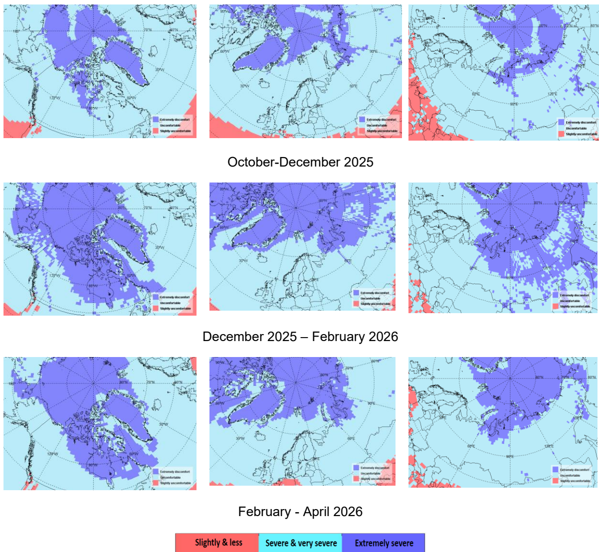
Figure 17a: Bodman's index (S) of weather severity for October 2025 – April 2026. Maps produced by the AARI. Data source: CCCS ERA5.
