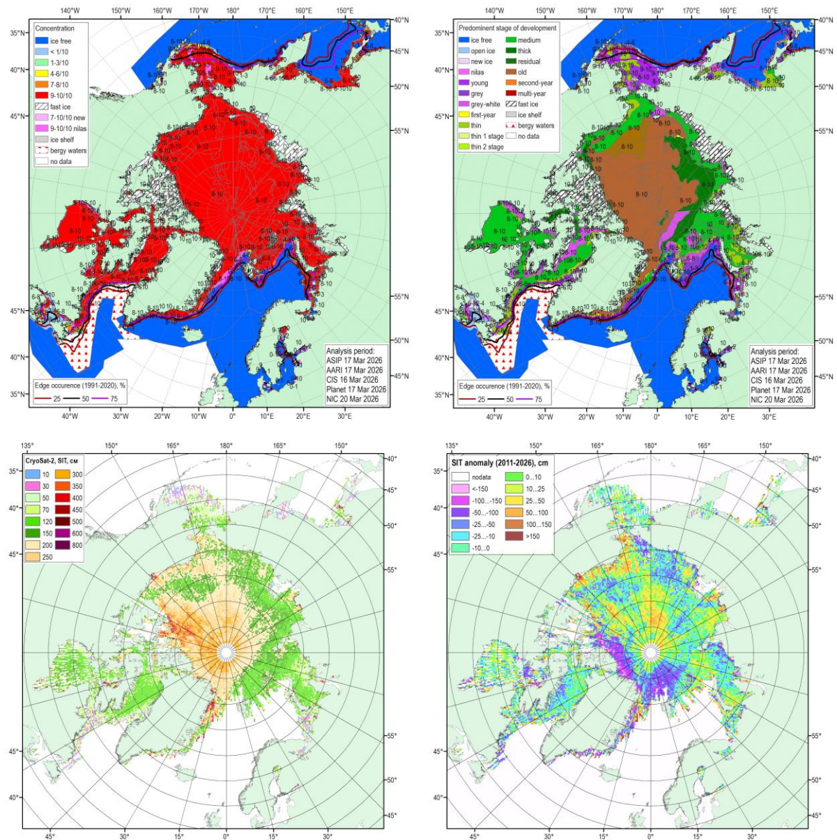
Figure 12: Blended Arctic sea-ice chart (AARI, ASIP, CIS, NIC, Planet) for 16-20 March 2026 and sea-ice edge occurrences for 16-20 March for 1991-2020 reference period (top), left top: total concentration, right top: predominant stage of development.; CryoSAT-2 sea-ice thickness (AWI v2p6) (bottom), bottom left: mean for March 2026, bottom right: anomaly for 2011-2026 reference period (bottom). Graphics produced by the AARI
