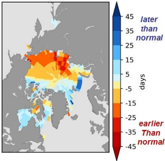
Figure 8: Forecast for the 2019 spring break-up where break-up is defined as the date when the ice concentration drops below 50%. Left: anomaly (difference from normal) based on the 2009-2017 period and right: the historical skill defined as the detrended anomaly correlation coefficient based on the 1981-2010 period.
