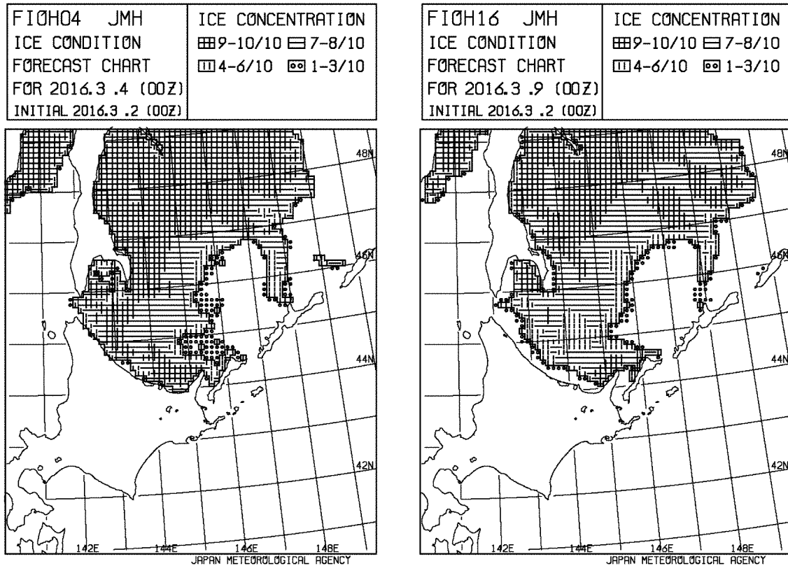
Figure VII-4 — Ice condition forecast charts for 4 and 9 March 2016 for the southern part of the Sea of Okhotsk (initial conditions for 2 March 2016)
