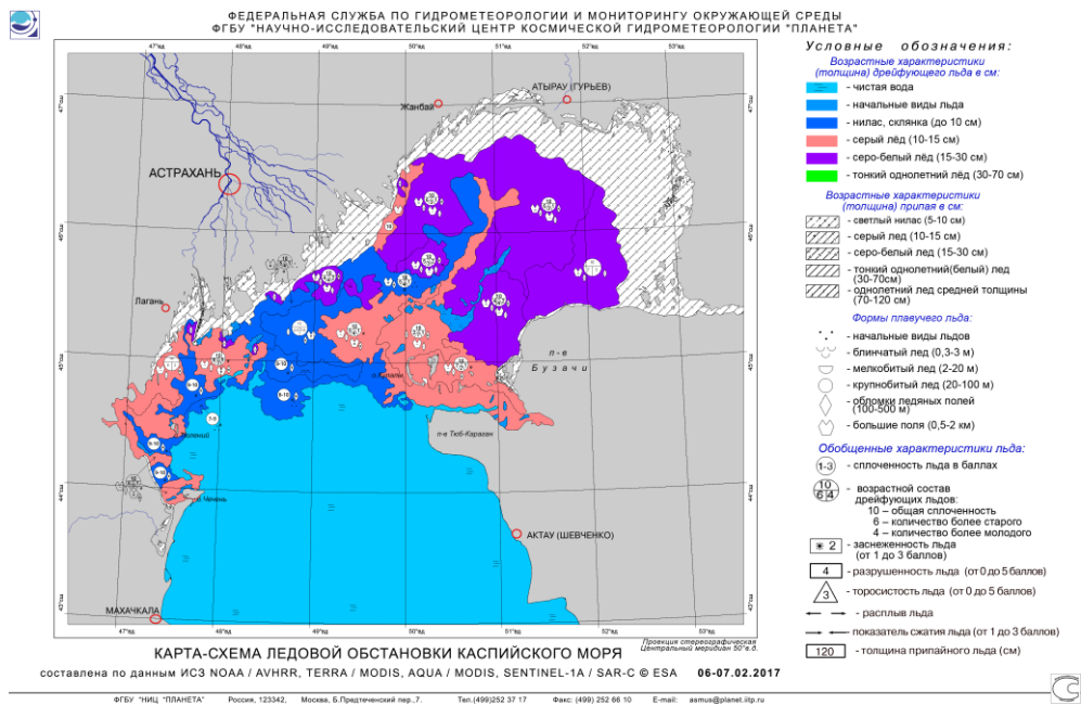
Figure III-6 – Planet ice chart in Russian national symbology for the Caspian Sea for 6-7 February 2017.
