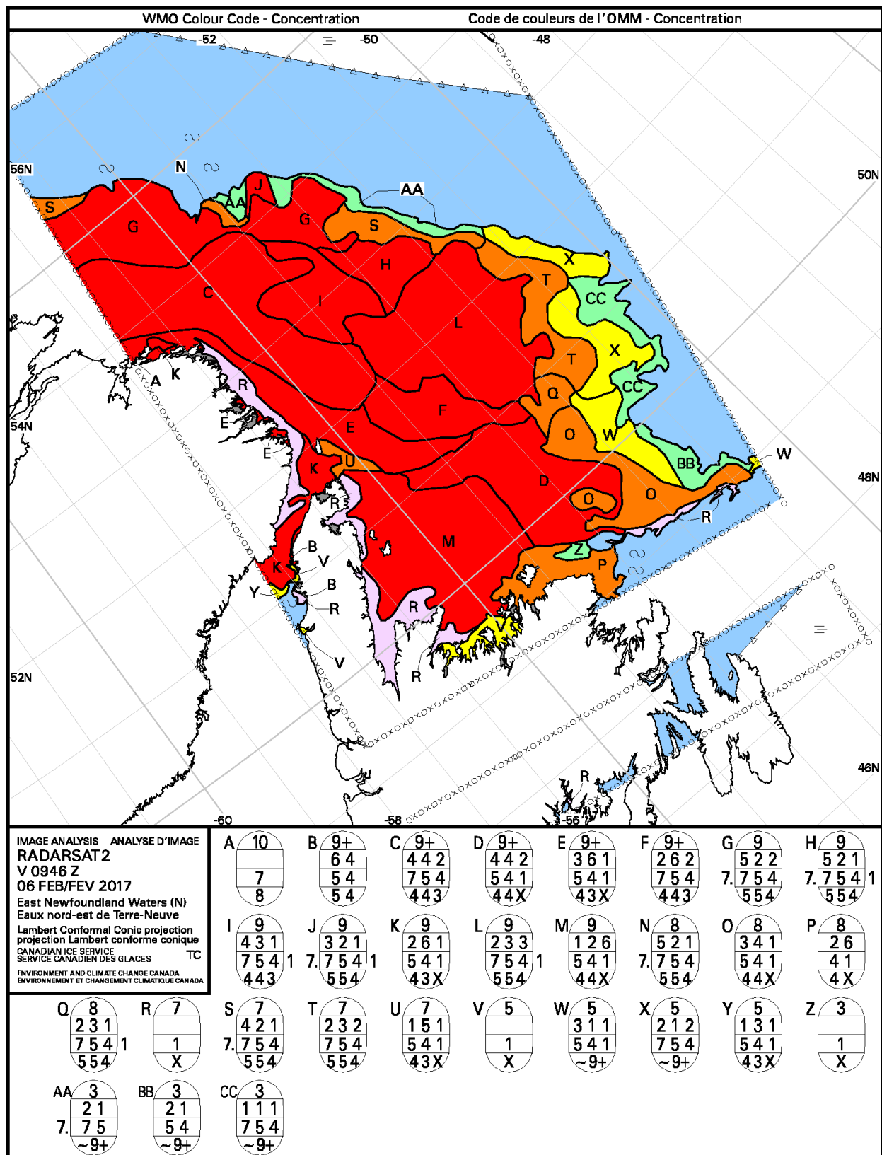
Figure XI-4 – Image analysis chart for East Newfoundland Waters on 06 February 2017
