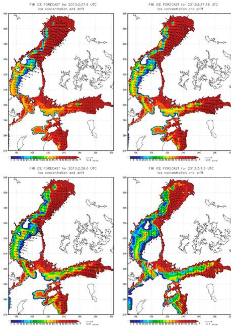
Figure VI-3 – Ice concentration and drift forecast for 27 th February – 1 st of March 2013 (t+3h, +12h, +24h and 48h)
