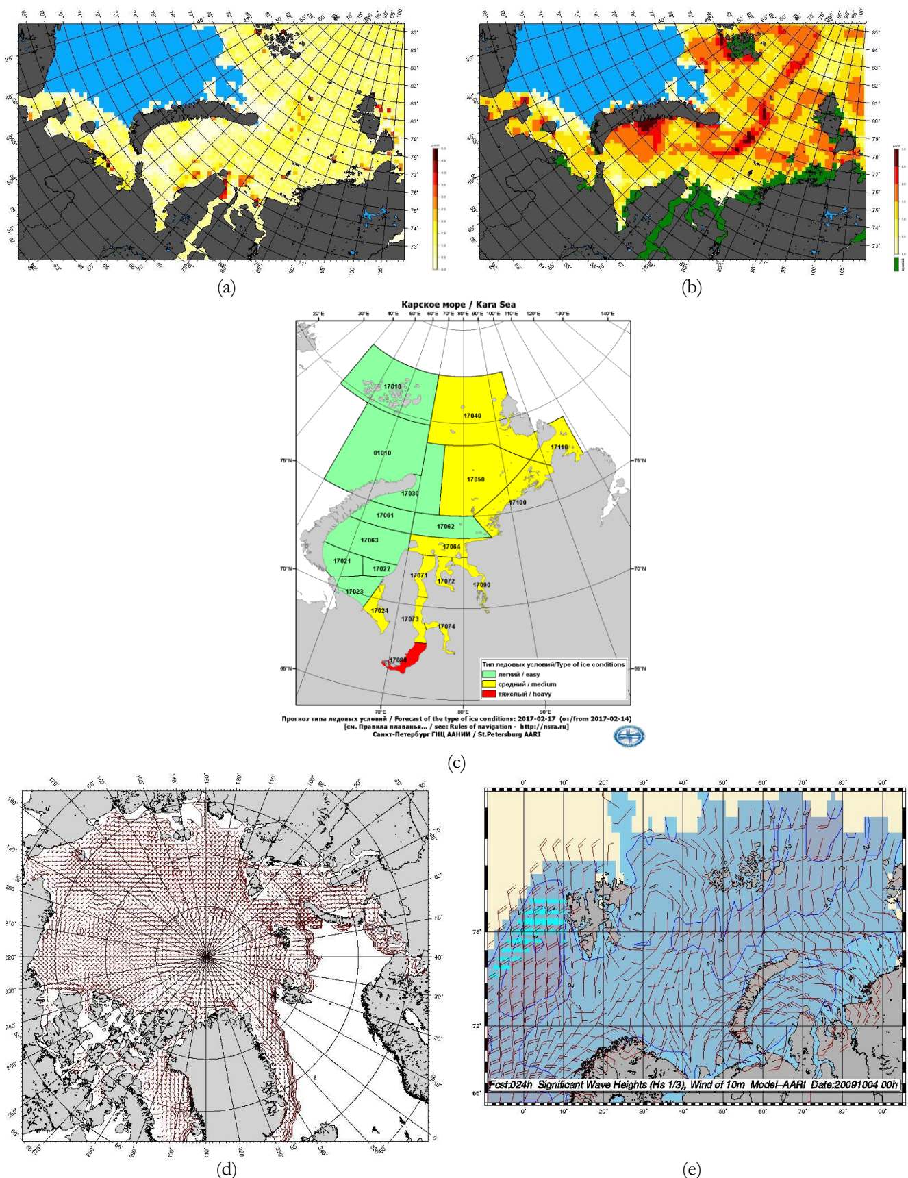
Figure III-8 – Short-term prognostic charts: 2010-02-05 +024h for the Barents-Kara Seas: hummocks concentration (a) and level of ice compacting (b); 2017-02-14 +72h: type of ice conditions (c); 2010-02-05 +024h for the Arctic Ocean: mean daily ice drift (d); 2009-10-03 +024h significant (3%) waves height, level of ice accretion and surface wind vectors for the Western Eurasian Arctic seas (e).
