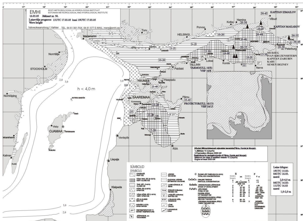
Figure V-1 – Ice chart for the Baltic proper for 16 March 2005.
