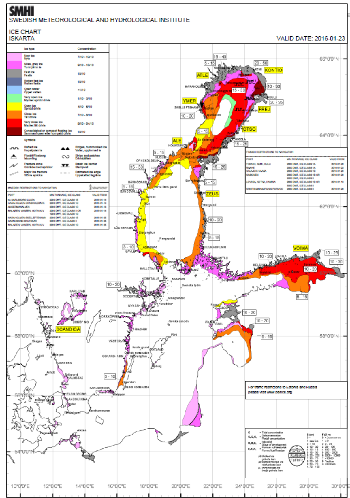
Figure X -1 – Daily ice chart for the Baltic Sea, 23 January 2016
