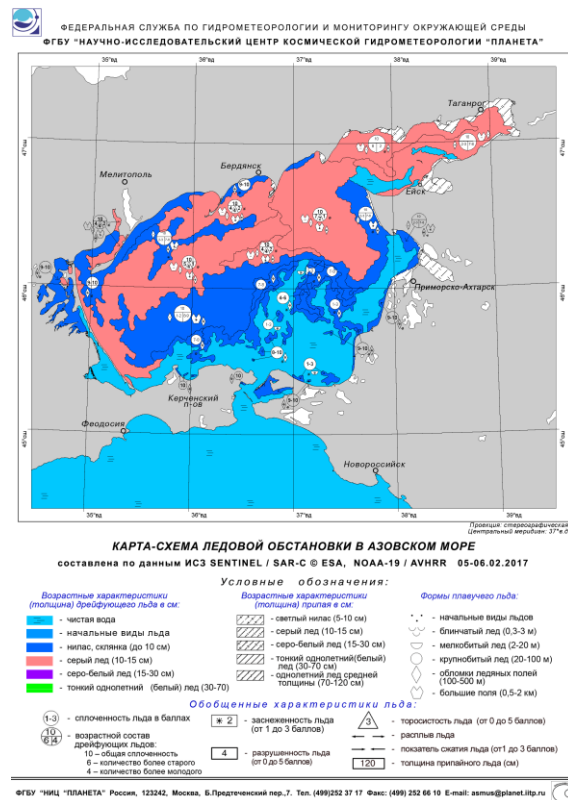
Figure III-5 – Planet ice chart in Russian national symbology for the Azov Sea for 5-6 February 2017.
