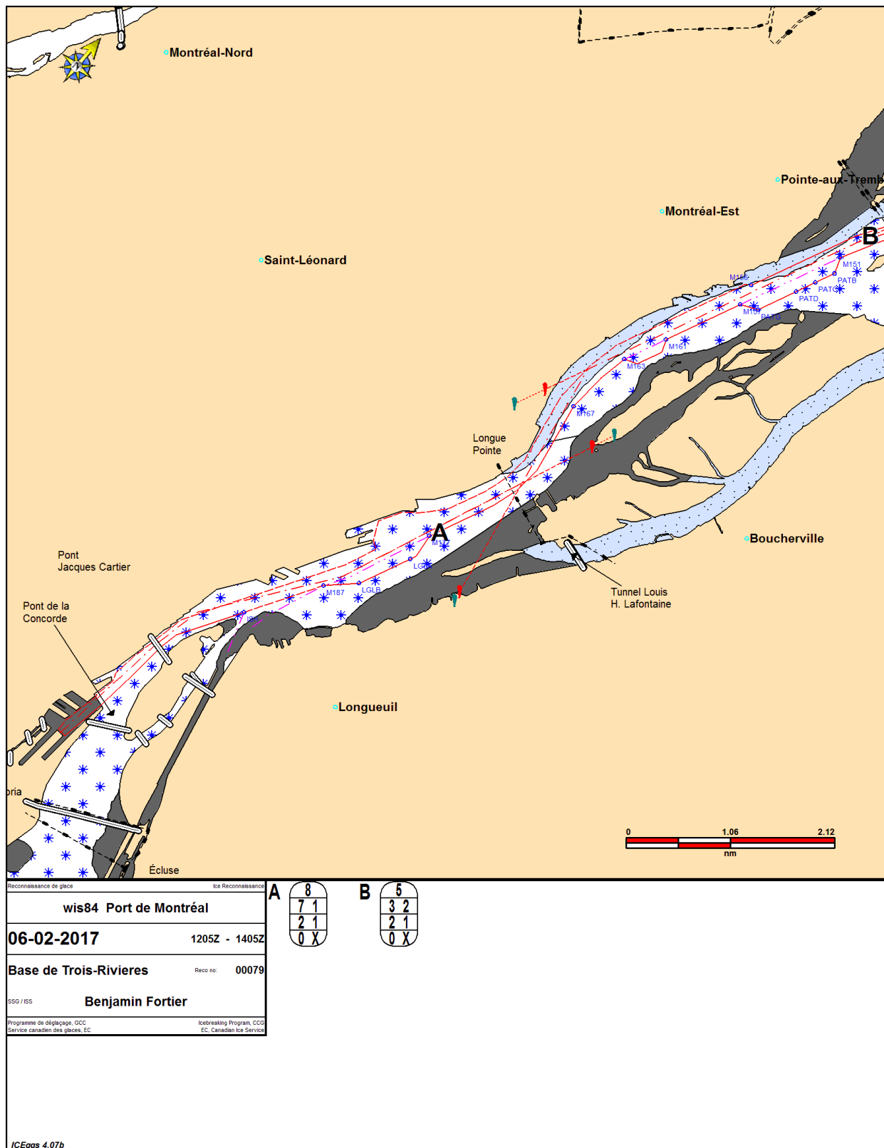
Figure XI-5 – Ice Reconnaissance chart for the Port of Montreal on 06 February 2017.
