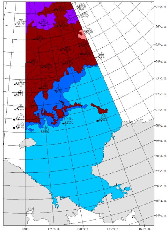
Figure III-4 – AARI ice chart in Russian national symbology for the Chukchi Sea for 3-4 October 2016
