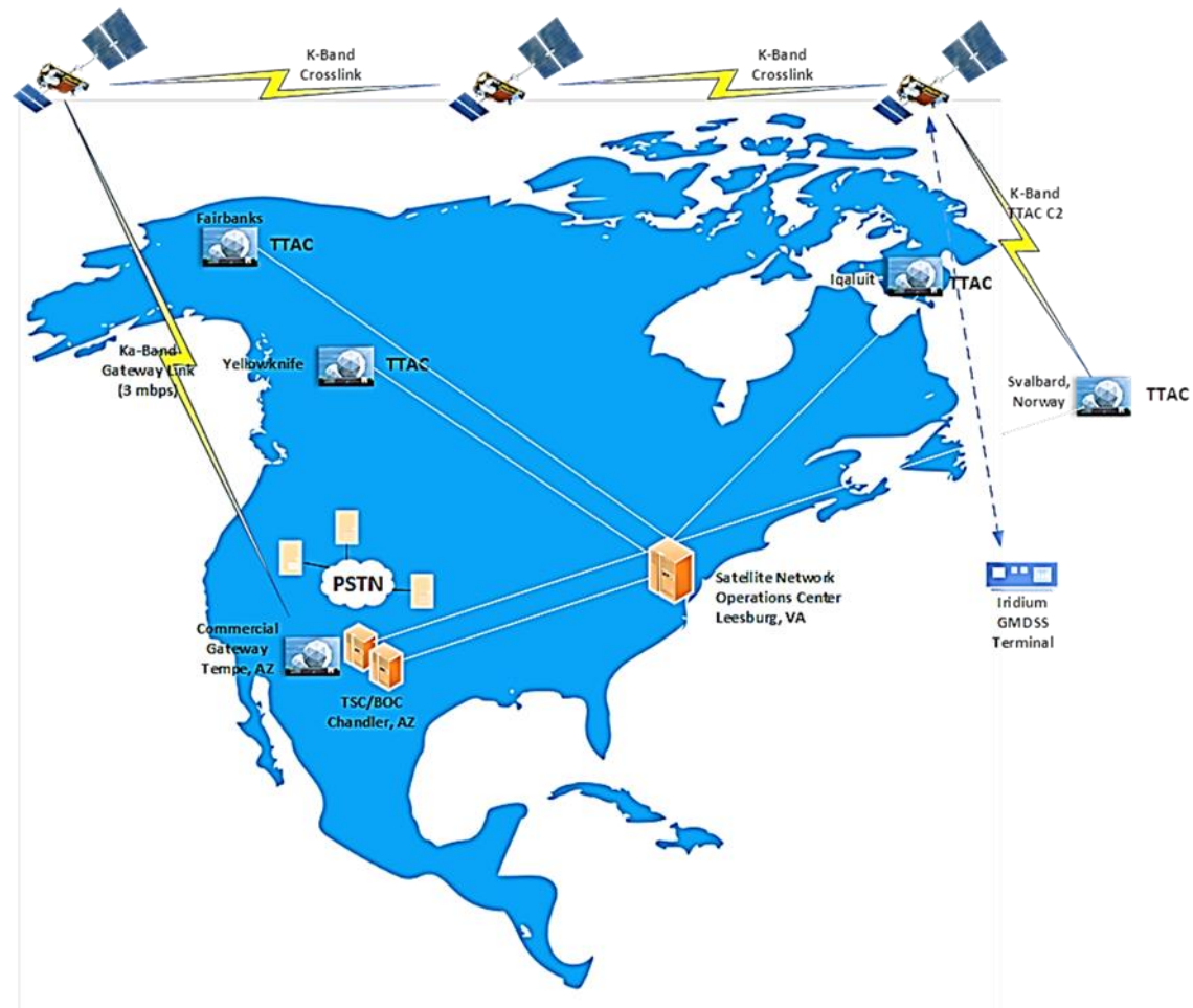
Figure 7 – The Iridium global satellite system, network overview (North and Central America)
